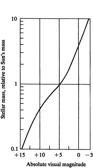
Figure 32. Absolute visual magnitude of main-sequence stars as a function of stellar mass.
