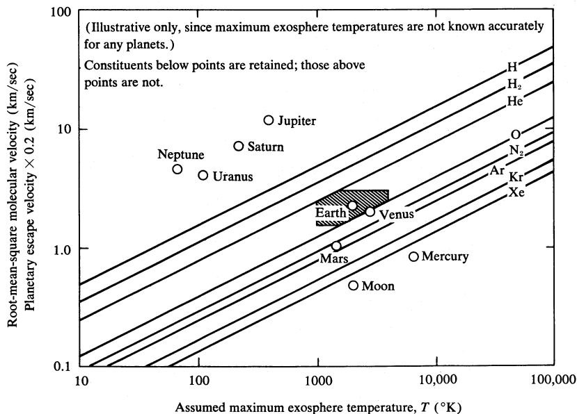
Figure 12. Planetary atmospheres.
