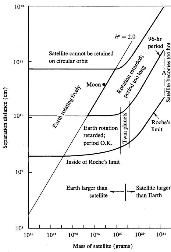
Figure 28. Hypothetical satellites of the Earth.
